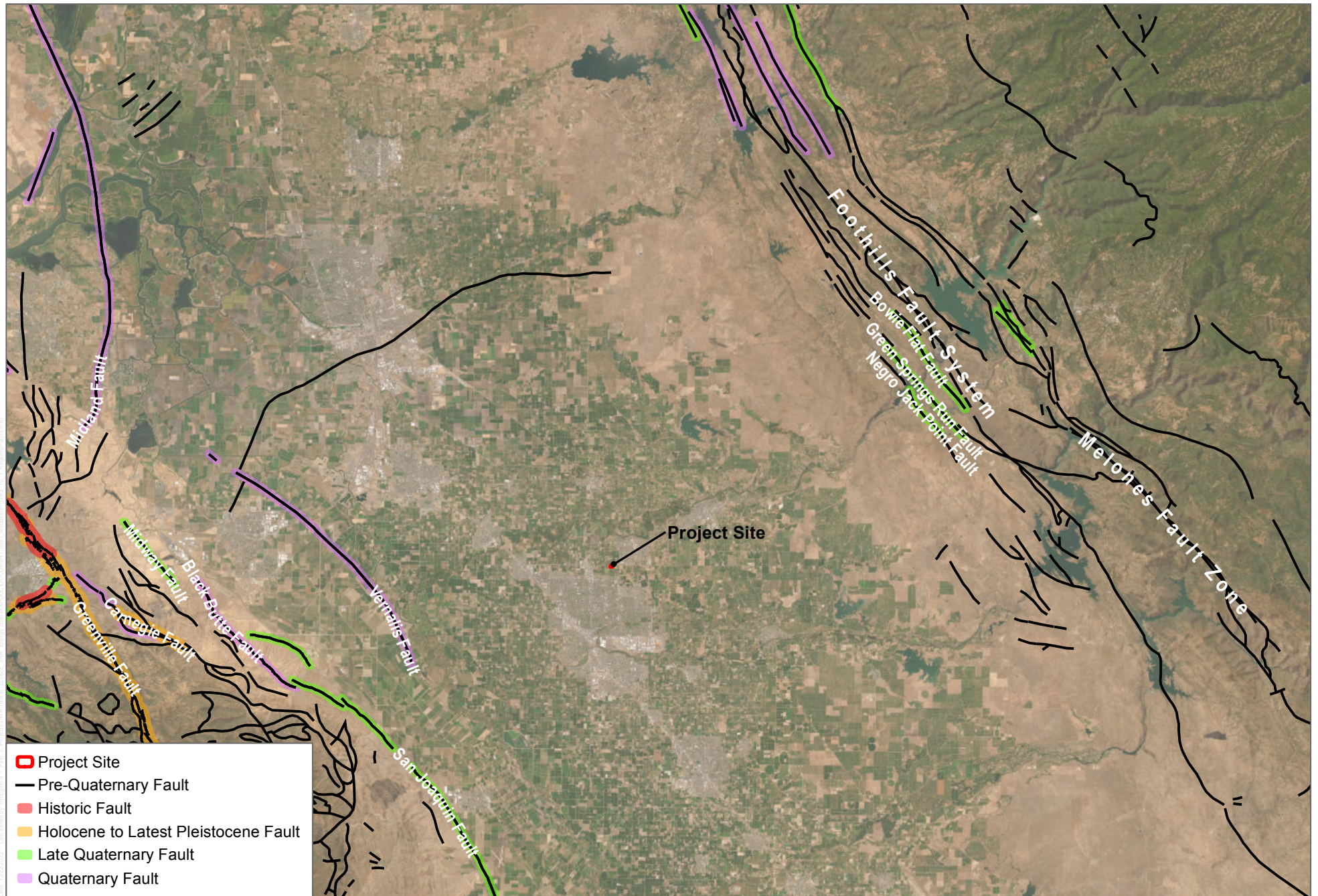
FIGURE 3.10-1 Regional Faults
