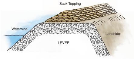
Figure 3: Sack topping on a levee
