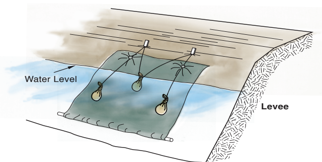
Figure 9: Waterside boil protection
