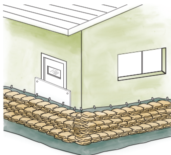
Figure 16: Structure protection
