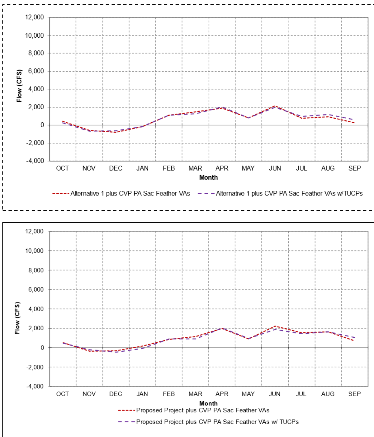
Figure 4I-I-5. Monthly Long-term (Top) and Critically Dry Water Year (Bottom) Average Qwest Flow for Alternative 1 Proposed Project plus CVP PA and Sacramento and Feather River VAs (with and without TUCPs)
