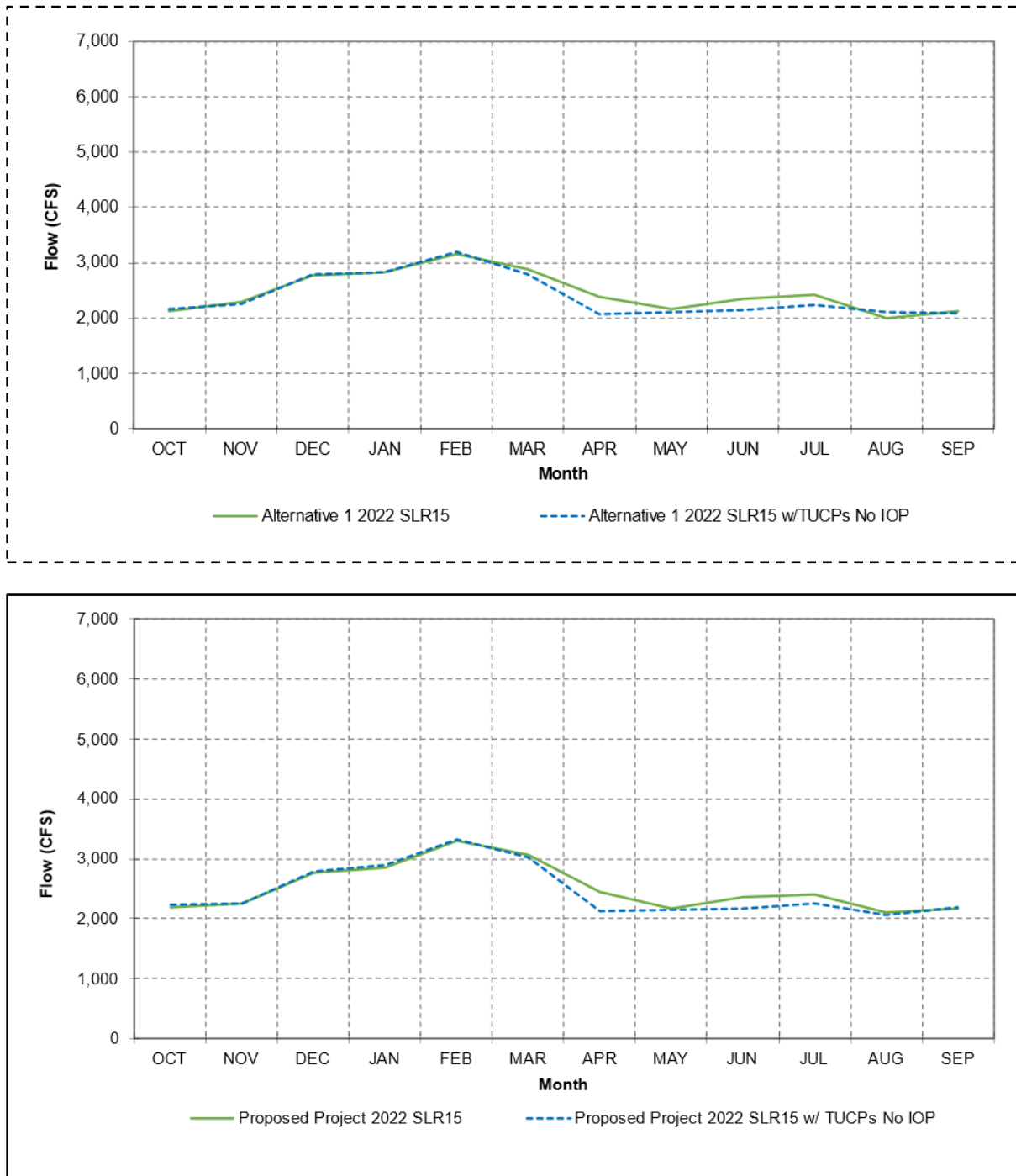
Figure 4I-I-12. Monthly Long-term (Top) and Critically Dry Water Year (Bottom) Average Georgiana Slough Flow for Alternative 1 the Proposed Project under Future Climate Centered around 2022 with 15 cm of Sea Level Rise (with and without TUCPs and the IOP)
