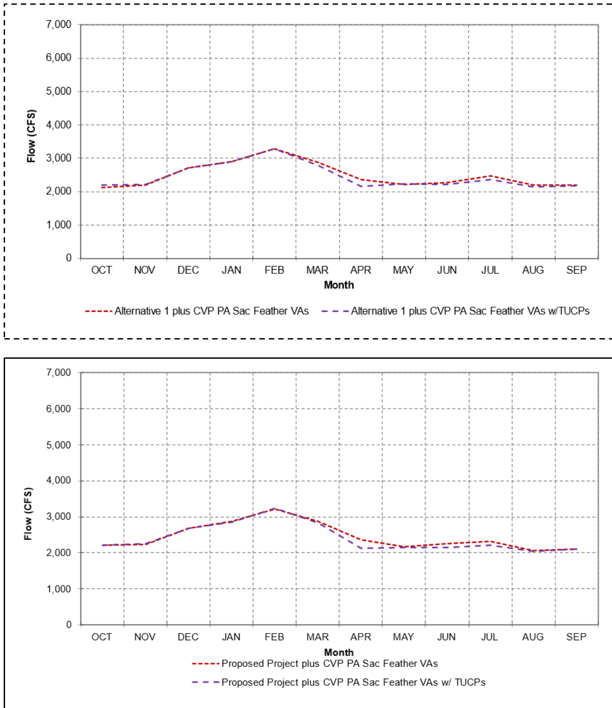
Figure 4I-I-3. Monthly Long-term (Top) and Critically Dry Water Year (Bottom) Average Georgiana Slough Flow for Alternative 1 Proposed Project plus CVP PA and Sacramento and Feather River VAs (with and without TUCPs)
