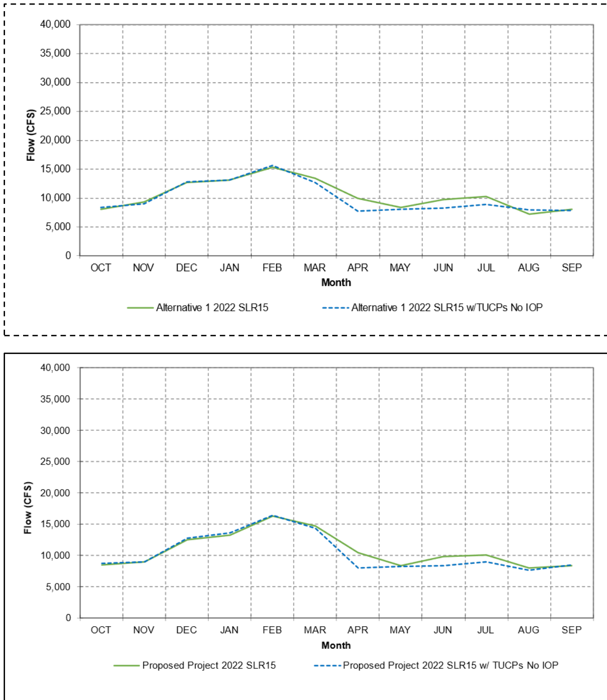
Figure 4I-I-10. Monthly Long-term (Top) and Critically Dry Water Year (Bottom) Average Sacramento River at Freeport Flow for Alternative 1 the Proposed Project under Future Climate Centered around 2022 with 15 cm of Sea Level Rise (with and without TUCPs and the IOP)
