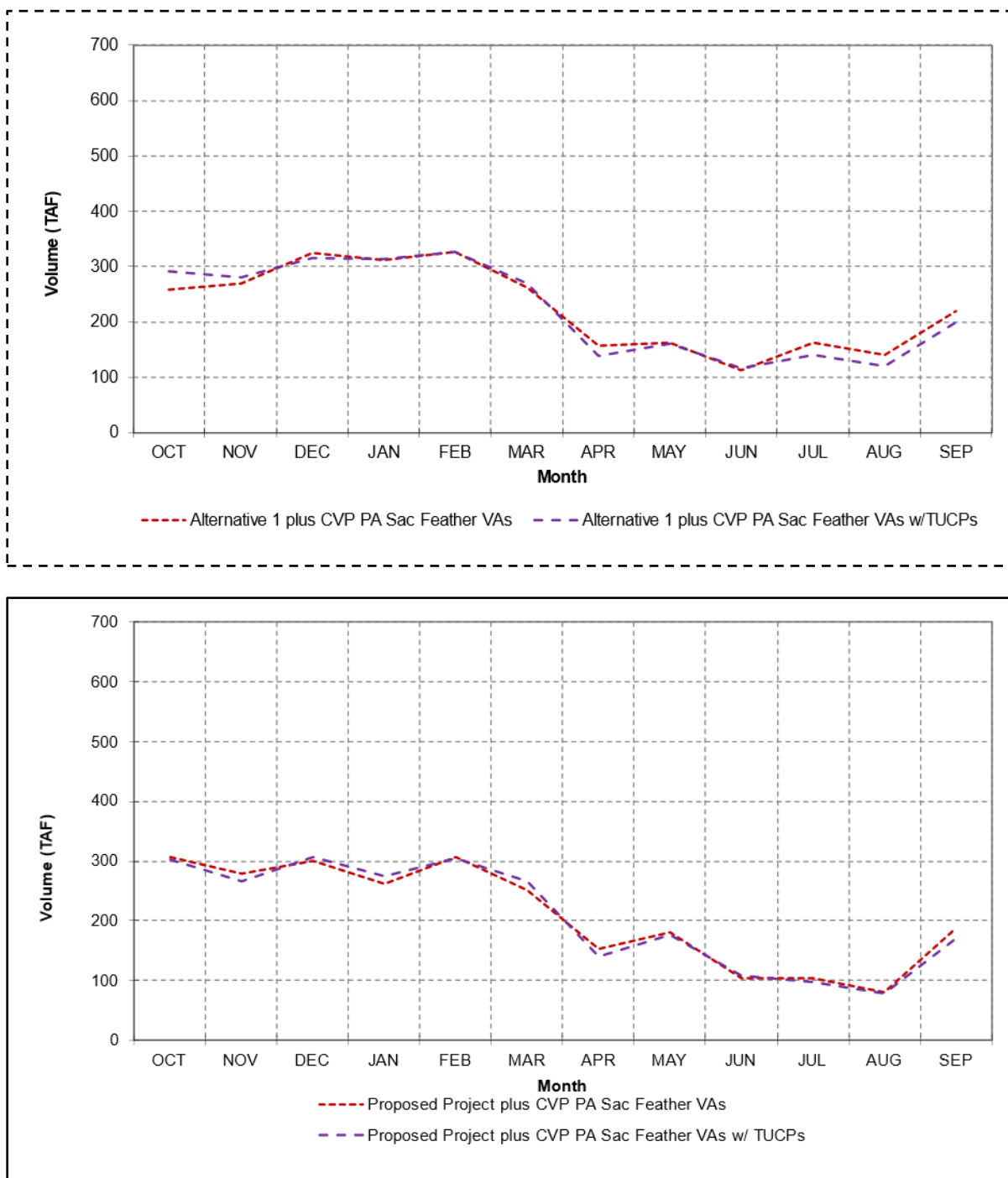
Figure 4I-I-8. Monthly Long-term (Top) and Critically Dry Water Year (Bottom) Average Delta Exports for Alternative 1 Proposed Project plus CVP PA and Sacramento and Feather River VAs (with and without TUCPs)
