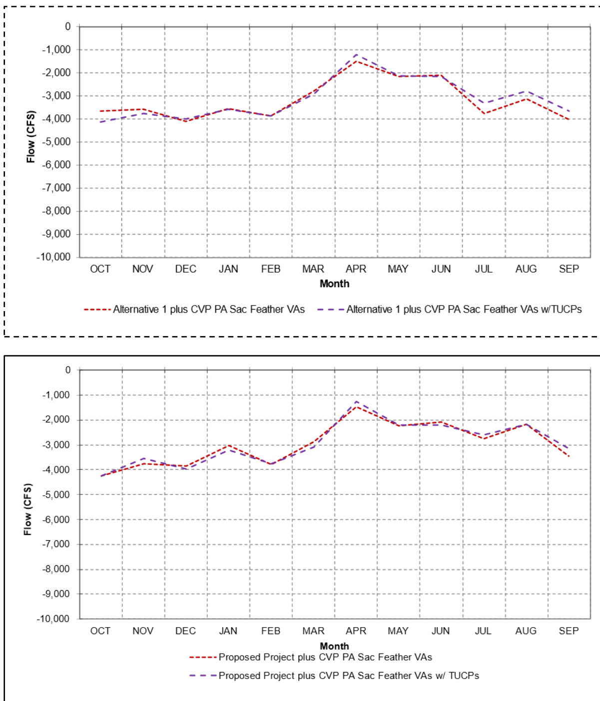
Figure 4I-I-7. Combined Old and Middle River Monthly Long-term (Top) and Critically Dry Water Year (Bottom) Average Flow for Alternative 1 Proposed Project plus CVP PA and Sacramento and Feather River VAs (with and without TUCPs)
