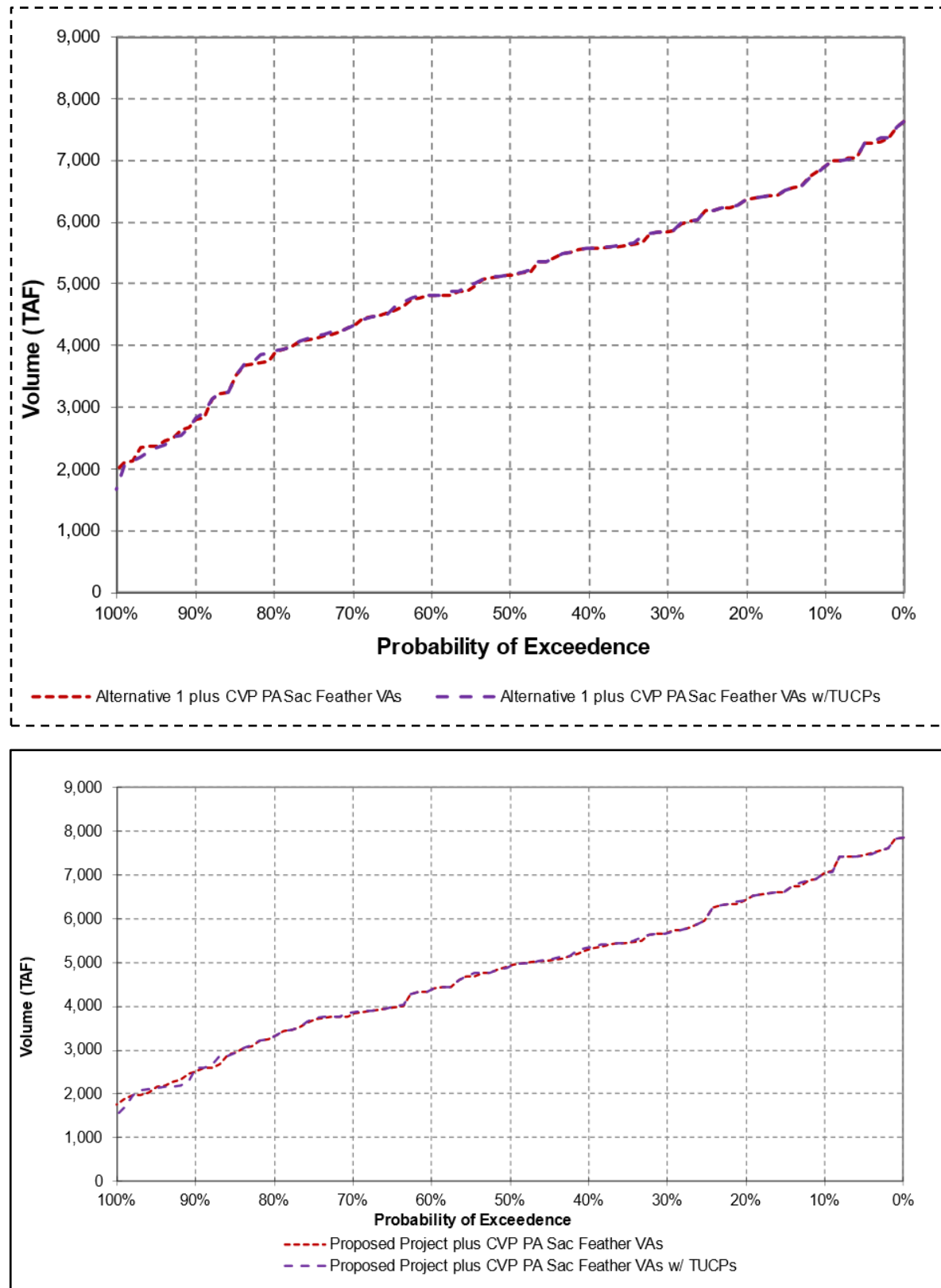
Figure 4I-I-9. Annual Delta Exports for Alternative 1 Proposed Project plus CVP PA and Sacramento and Feather River VAs (with and without TUCPs)
