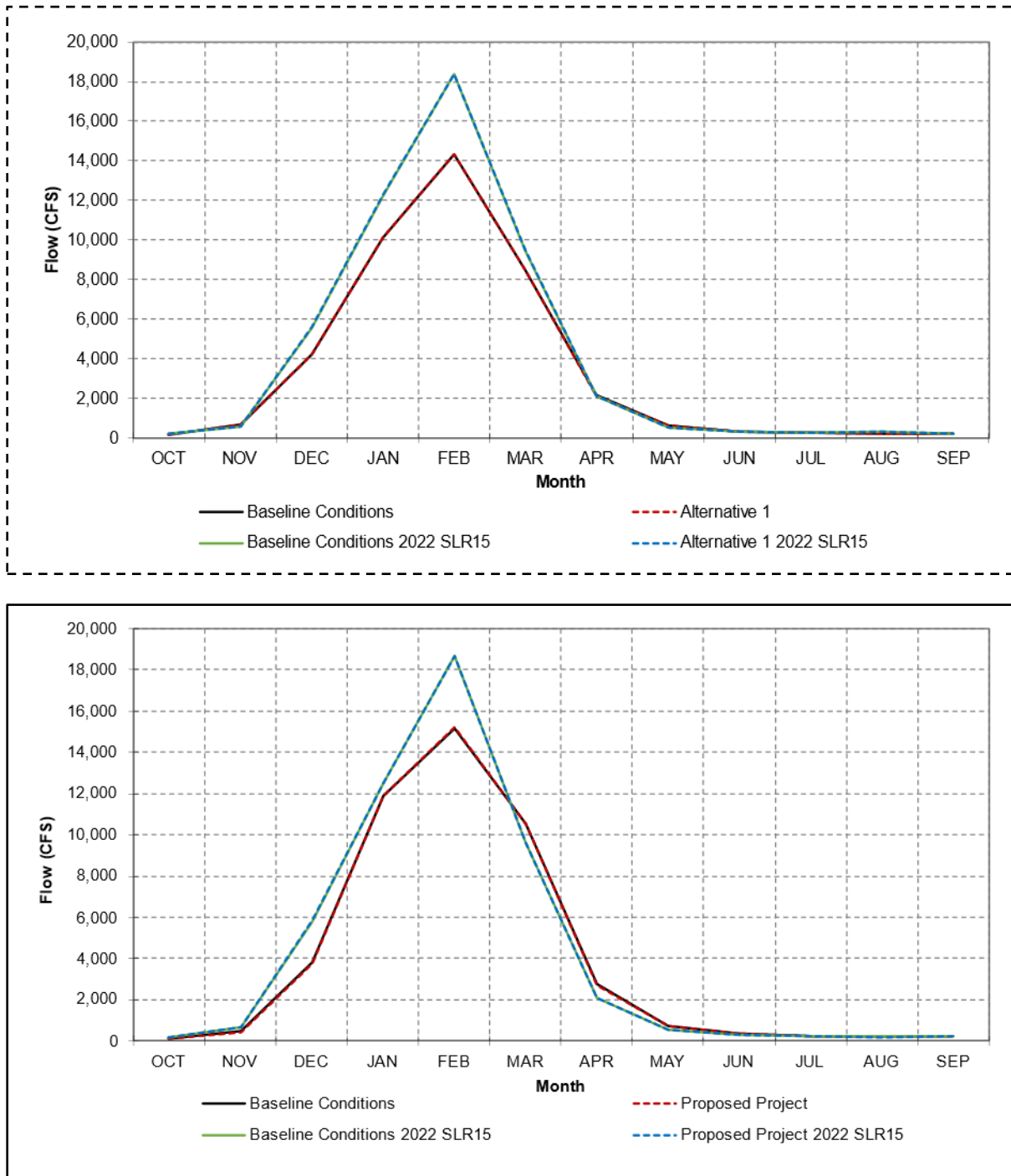
Figure 4D-2. Monthly Long-term Average Yolo Bypass Flow for the Baseline Conditions and Alternative 1 Proposed Project under Adjusted Historical Hydrology and Future Climate Centered around 2022 with 15 cm of Sea Level Rise
