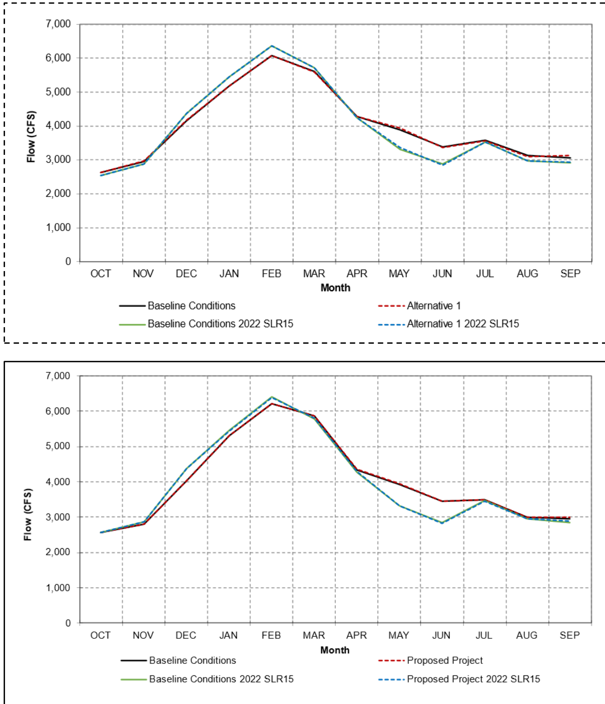
Figure 4D-3. Monthly Long-term Average Georgiana Slough Flow for the Baseline Conditions and Alternative-1 Proposed Project under Adjusted Historical Hydrology and Future Climate Centered around 2022 with 15 cm of Sea Level Rise
