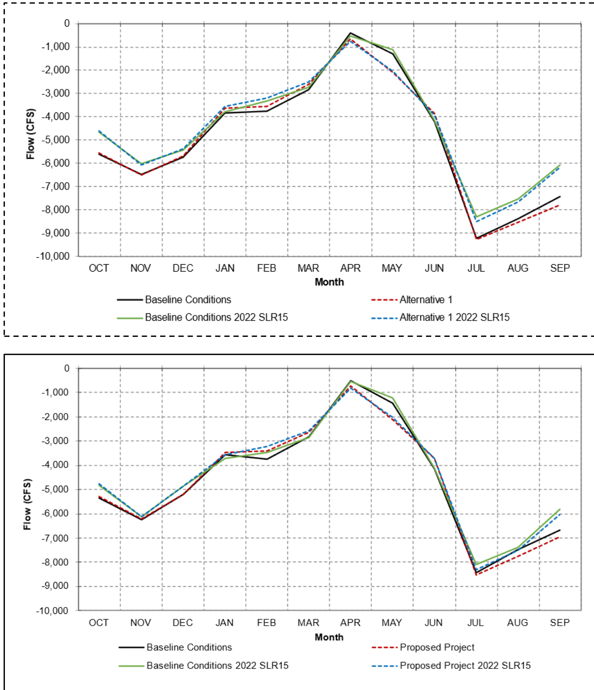
Figure 4D-7. Combined Old and Middle River Monthly Long-term Average Flow for the Baseline Conditions and Alternative 1 Proposed Project under Adjusted Historical Hydrology and Future Climate Centered around 2022 with 15 cm of Sea Level Rise
