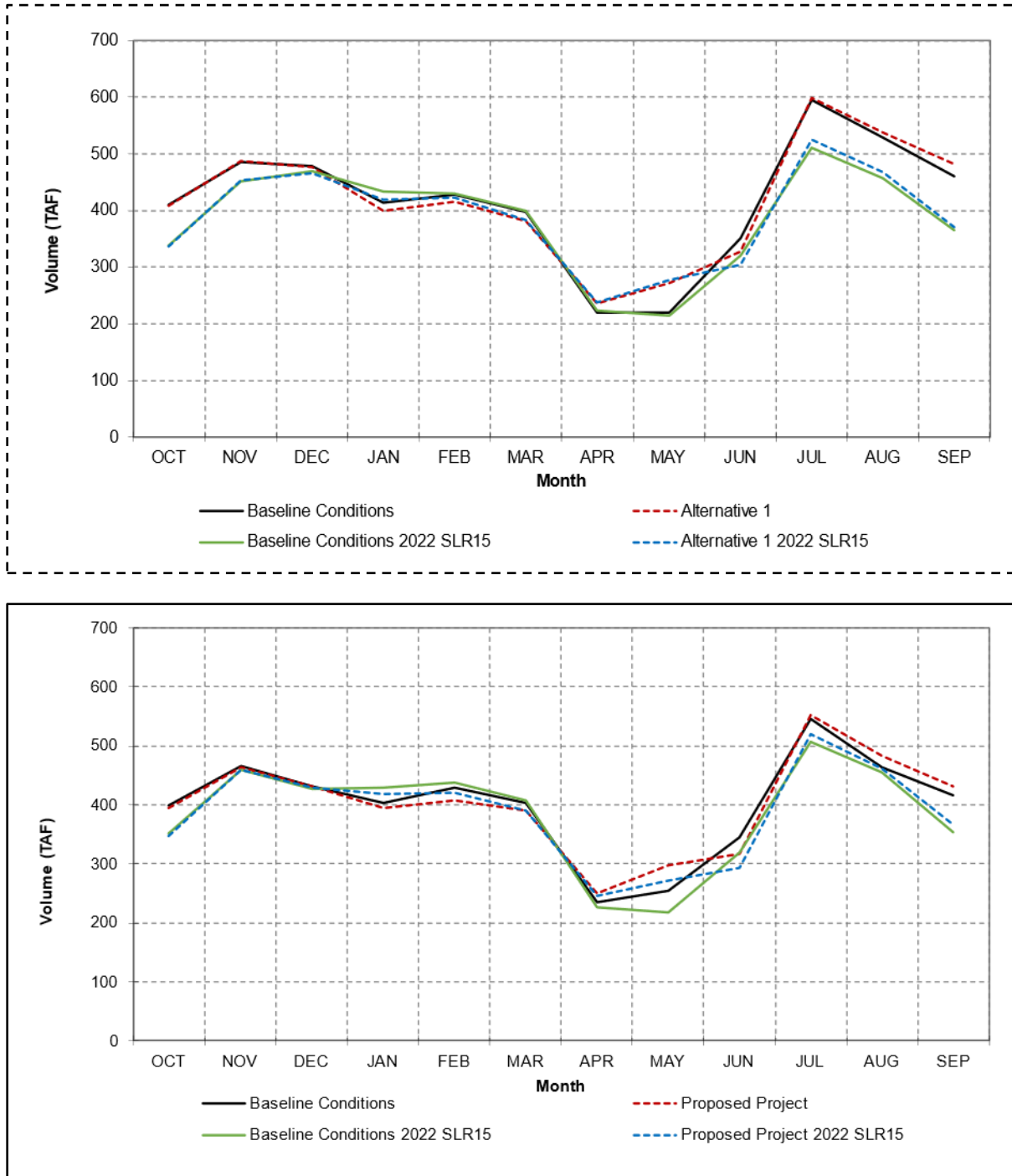
Figure 4D-8. Monthly Long-term Average Delta Exports for the Baseline Conditions and Alternative-1 Proposed Project under Adjusted Historical Hydrology and Future Climate Centered around 2022 with 15 cm of Sea Level Rise
