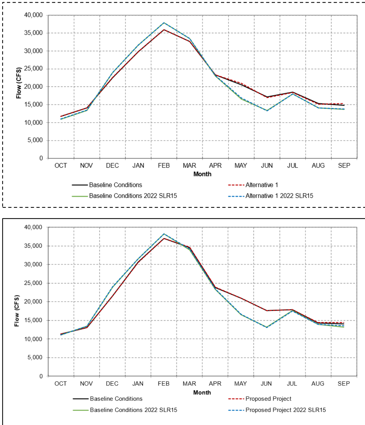
Figure 4D-1. Sacramento River at Freeport Monthly Long-term Average Flow for the Baseline Conditions and Alternative 1 Proposed Project under Adjusted Historical Hydrology and Future Climate Centered around 2022 with 15 cm of Sea Level Rise
