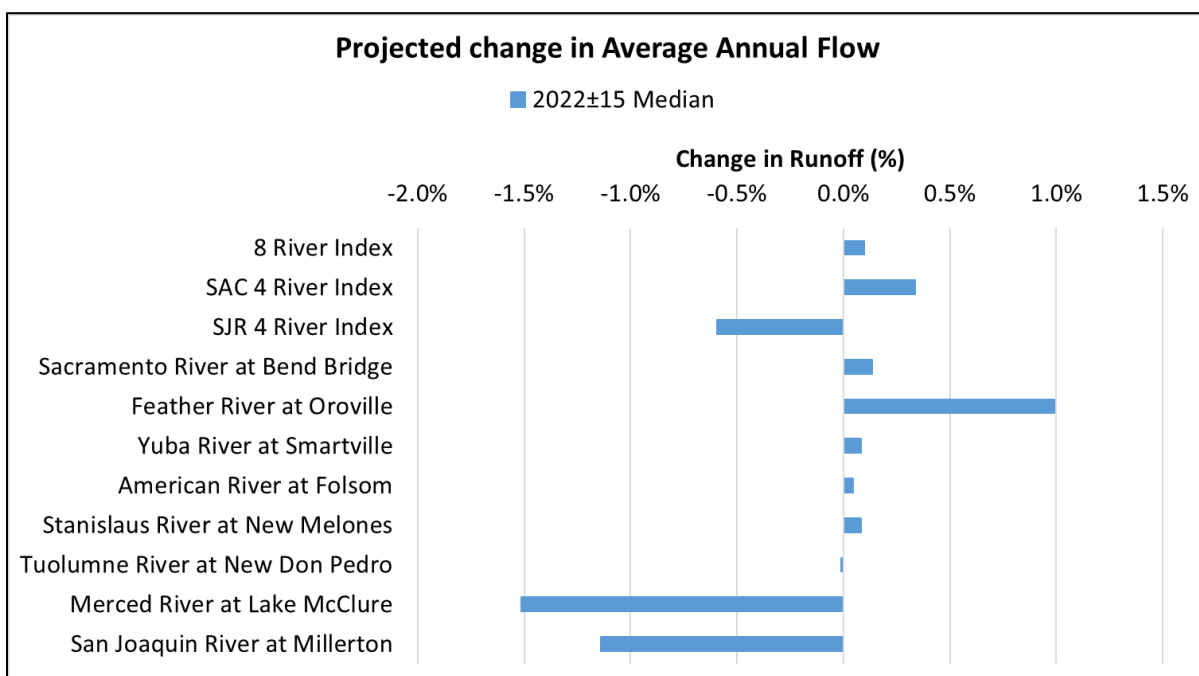
Figure 4D-4. Projected Changes in Runoff for Major Watersheds in the Sacramento and San Joaquin River Basins for 2022±15 Median Climate Change Scenario
