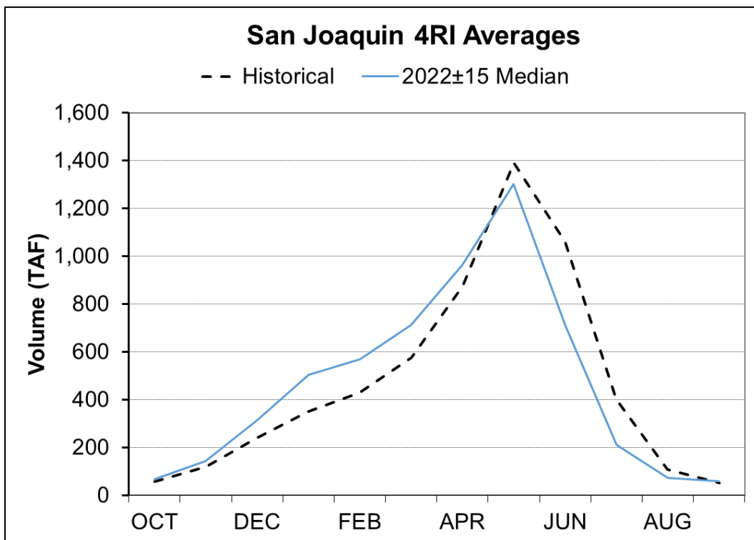
Figure 4D-5. Projected Changes in Monthly Pattern of Runoff for the Sacramento Basin ( left top ) and San Joaquin Basin ( right bottom ) for 2022±15 Median Climate Change Scenario.
