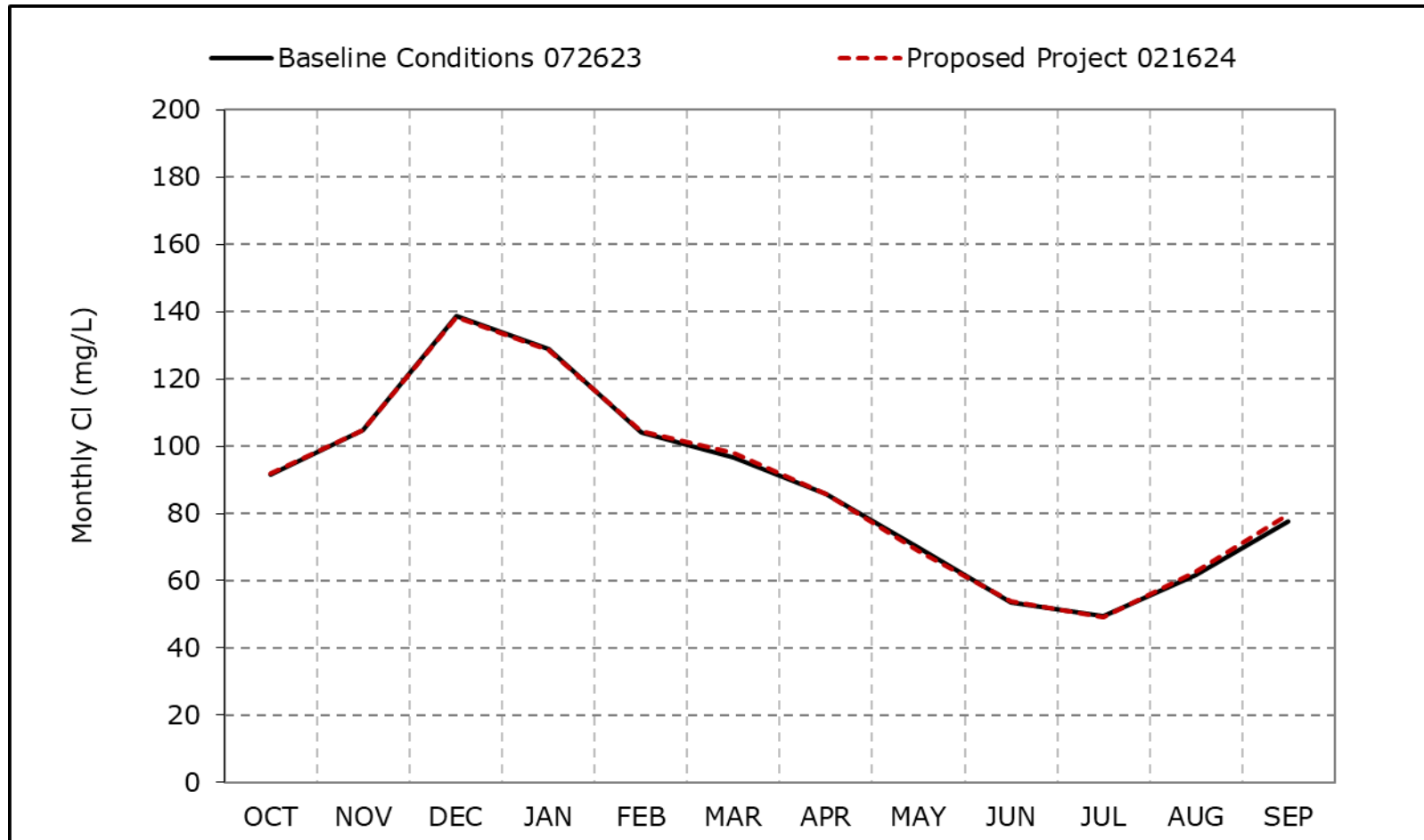
Figure 4B-7-12a. Jones Pumping Plant South Delta Exports Chloride, Long-Term Average Cl
