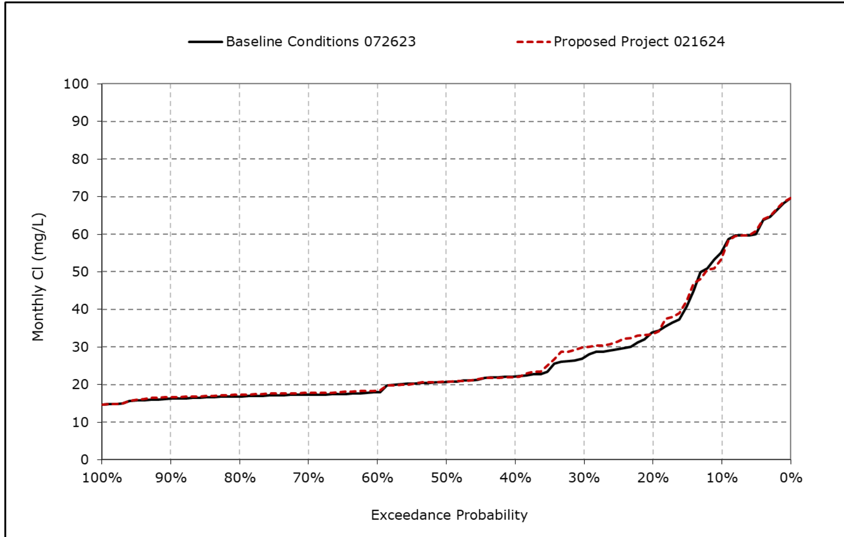
Figure 4B-7-2q. Sacramento River at Rio Vista Chloride, August Cl
