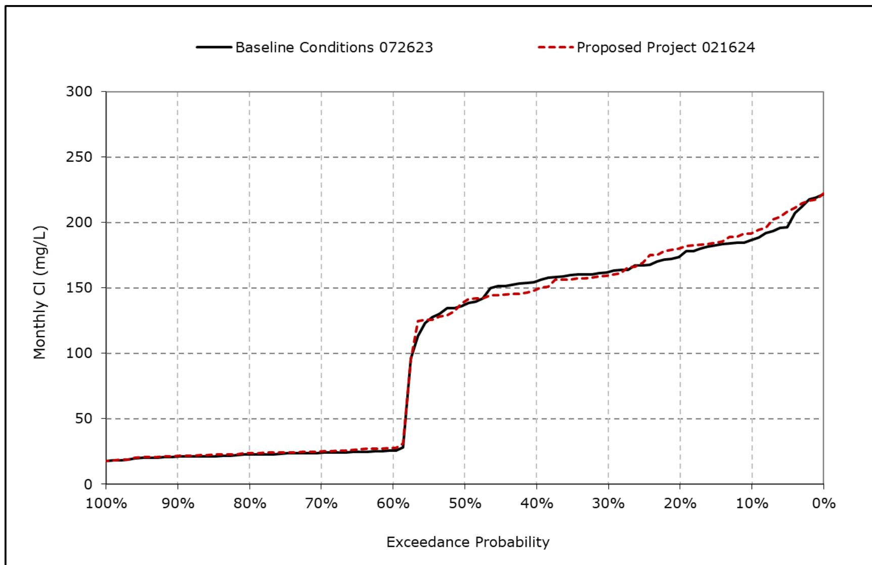
Figure 4B-7-9g. Contra Costa Pumping Plant Chloride, October Cl
