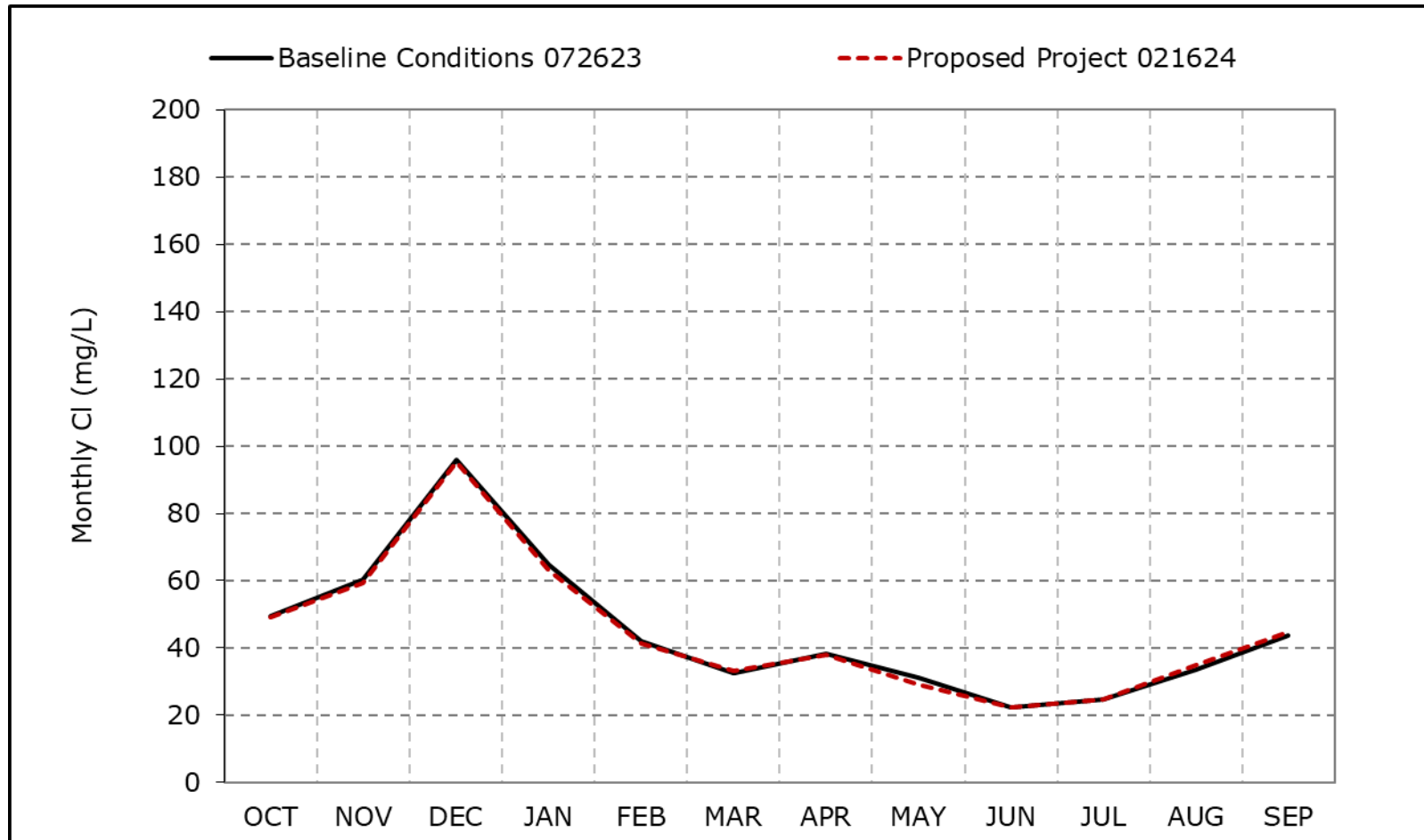
Figure 4B-7-6a. San Joaquin River at Prisoners Point Chloride, Long-Term Average CI
