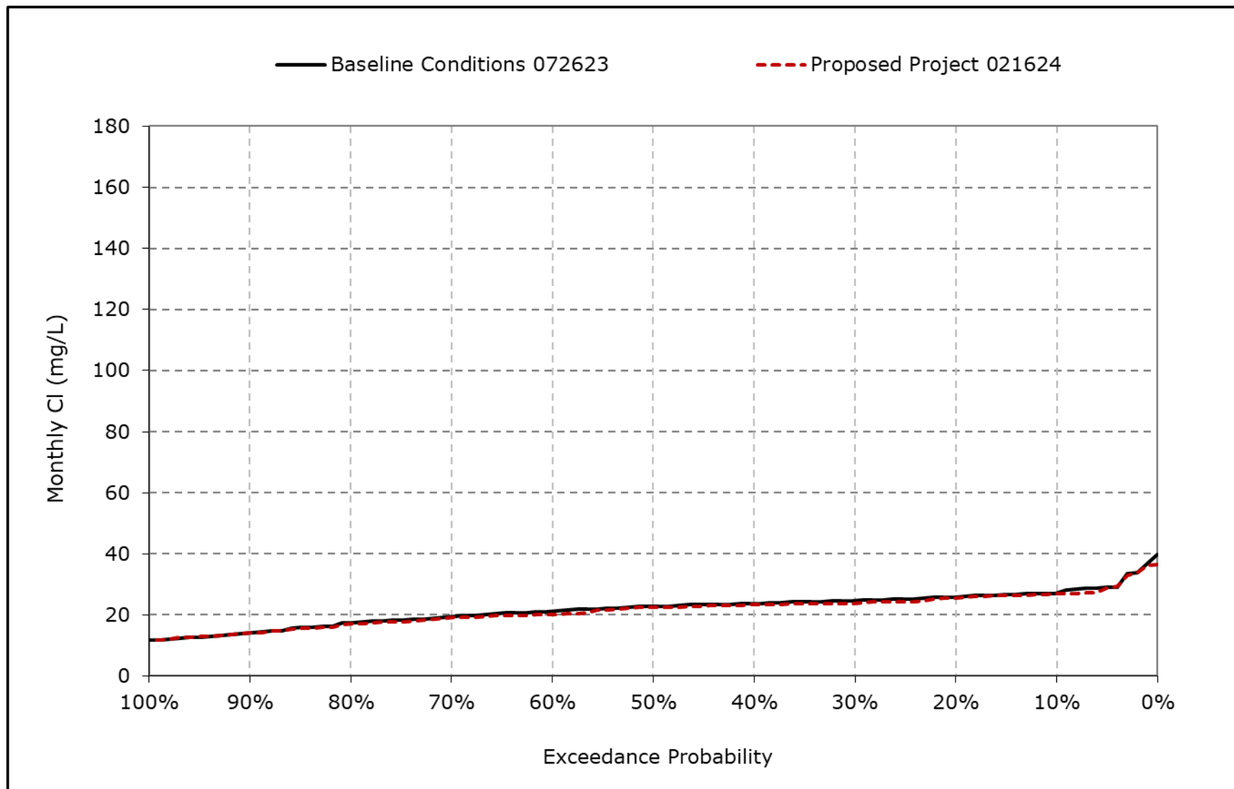
Figure 4B-7-5n. San Joaquin River at San Andreas Chloride, May CI
