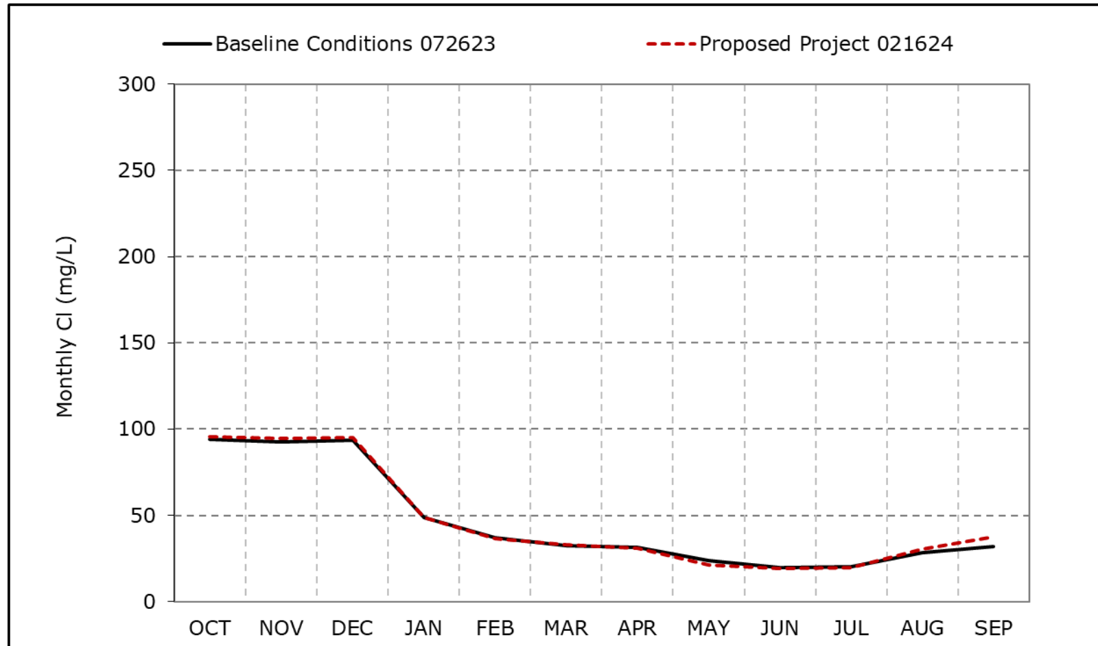
Figure 4B-7-9b. Contra Costa Pumping Plant Chloride, Wet Year Average CI
