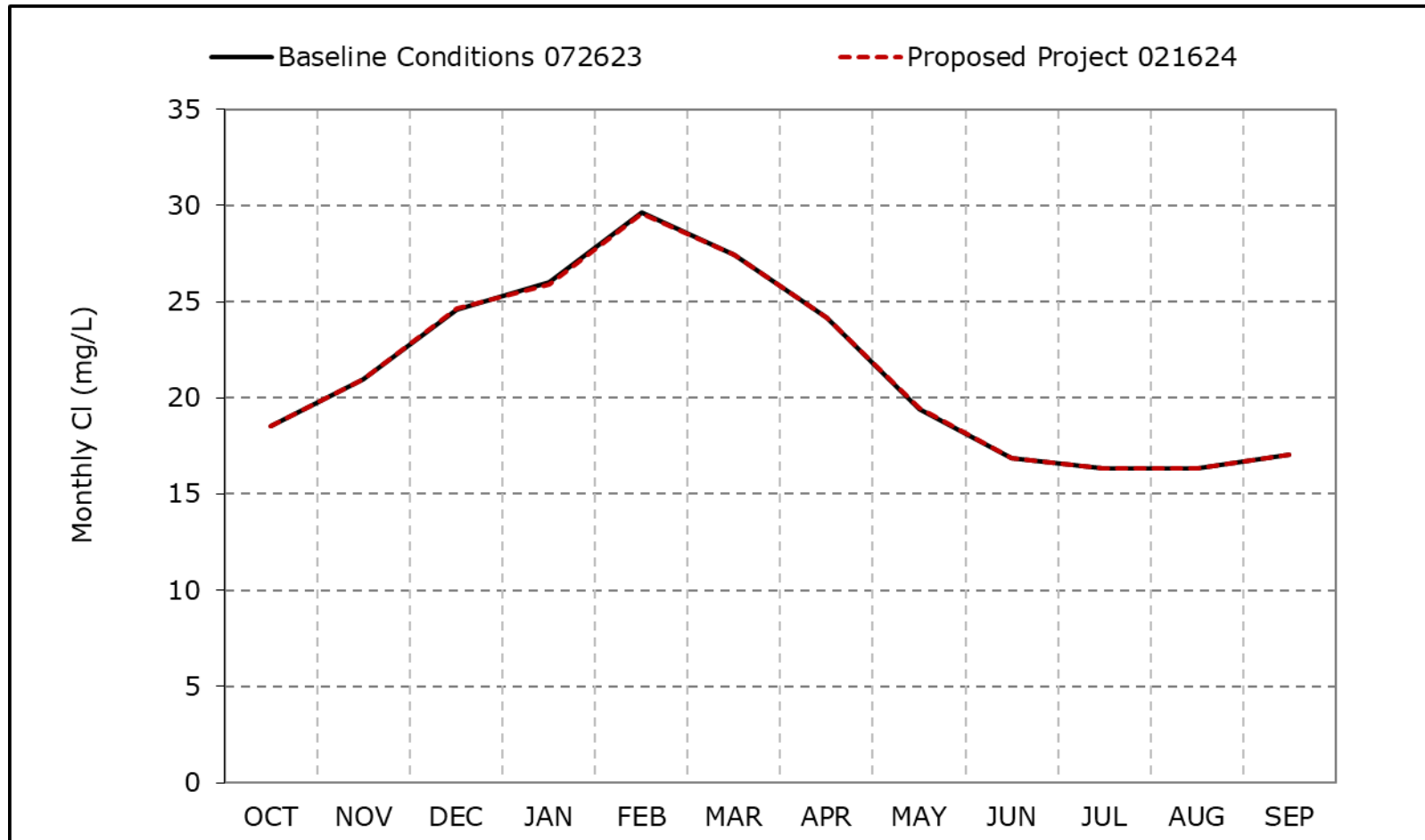
Figure 4B-7-13c. North Bay Aqueduct Chloride, Above Normal Year Average Cl
