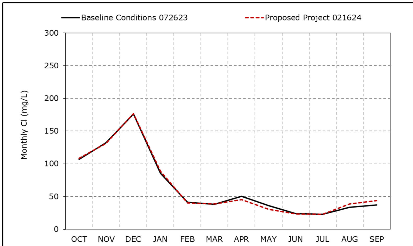
Figure 4B-7-9c. Contra Costa Pumping Plant Chloride, Above Normal Year Average CI
