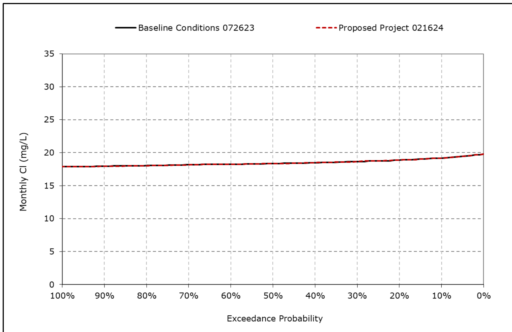
Figure 4B-7-13g. North Bay Aqueduct Chloride, October CI
