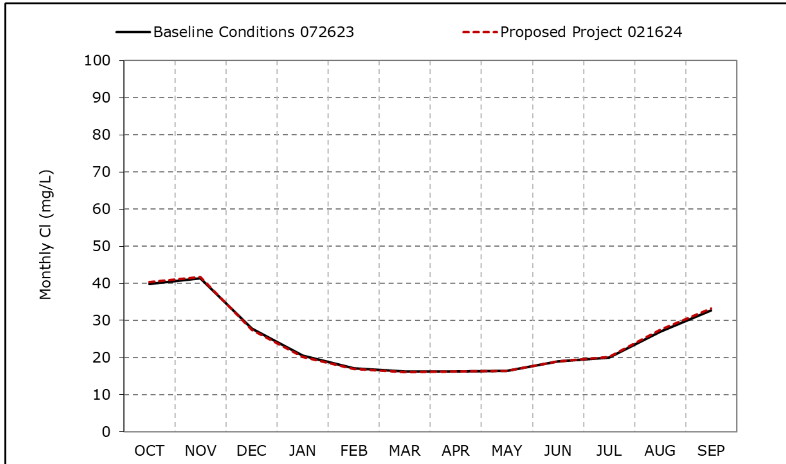
Figure 4B-7-2a. Sacramento River at Rio Vista Chloride, Long-Term Average Cl
