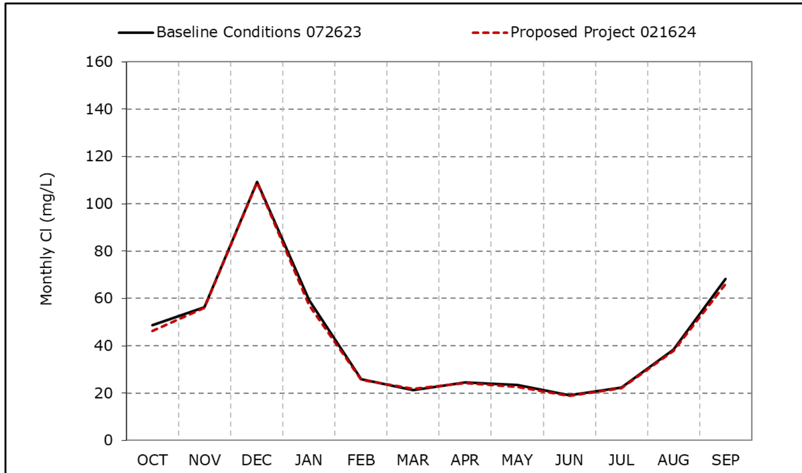
Figure 4B-7-5d. San Joaquin River at San Andreas Chloride, Below Normal Year Average Cl
