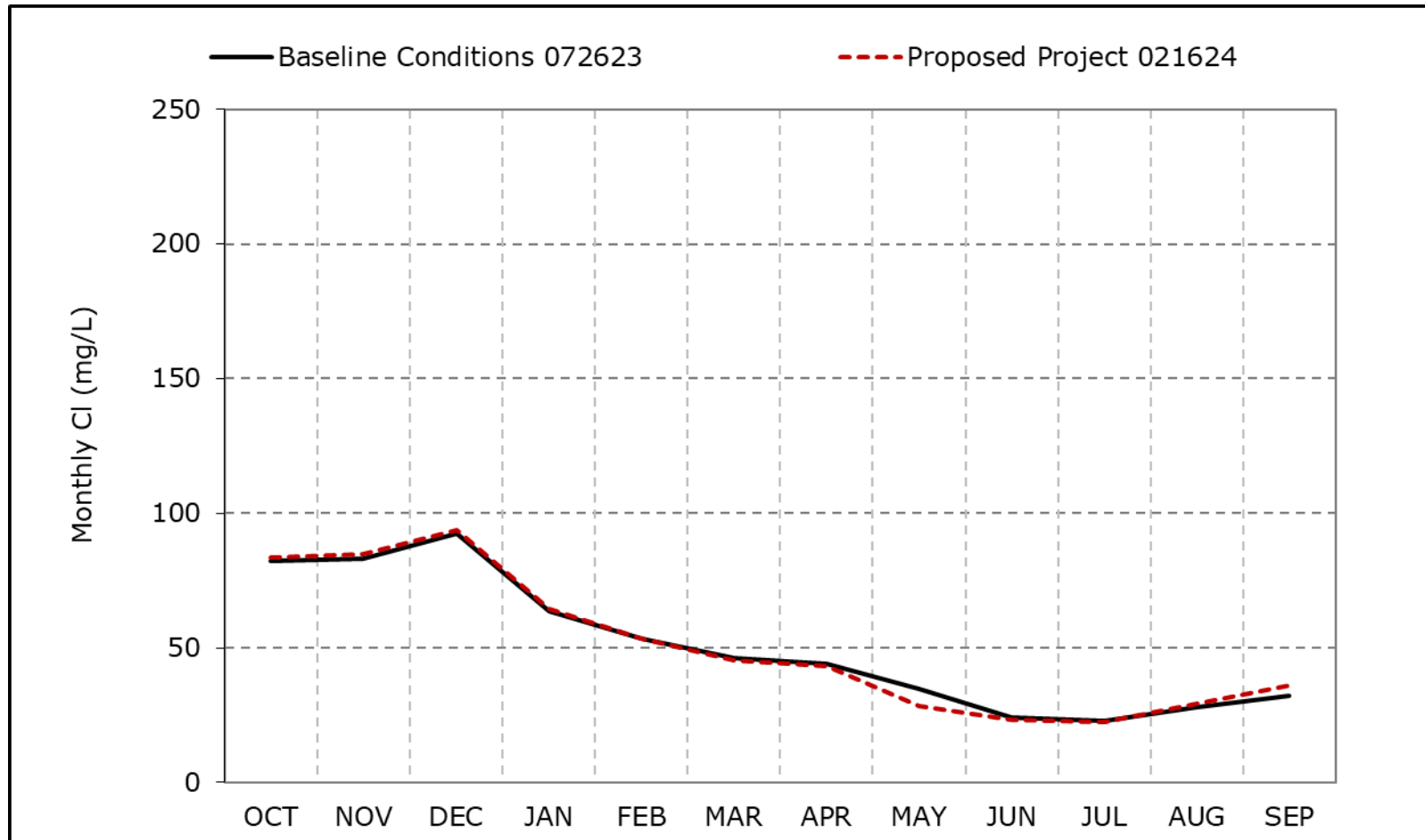
Figure 4B-7-7b. Old River at Highway 4 Chloride, Wet Year Average Cl
