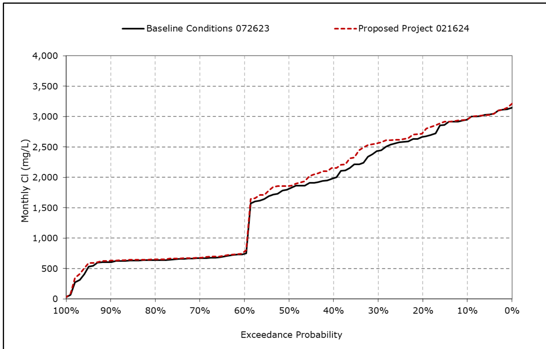
Figure 4B-7-3r. Sacramento River at Collinsville Chloride, September Cl
