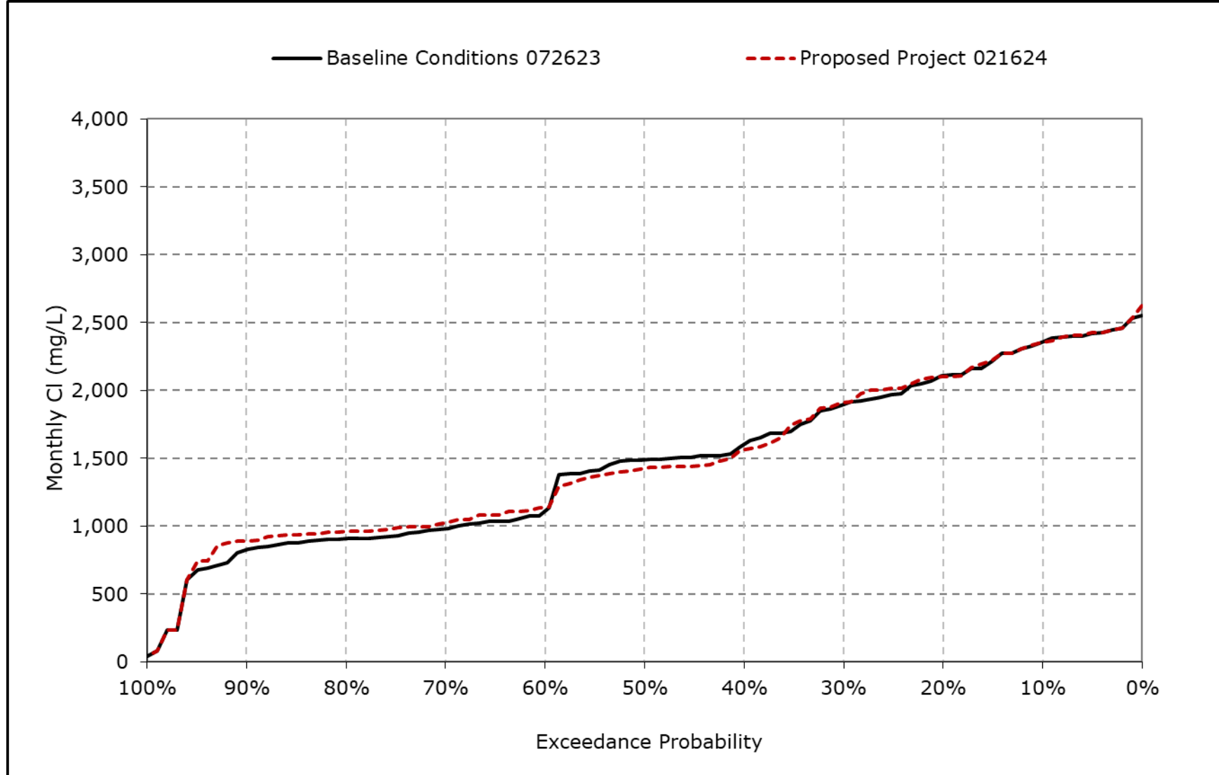
Figure 4B-7-3q. Sacramento River at Collinsville Chloride, August Cl
