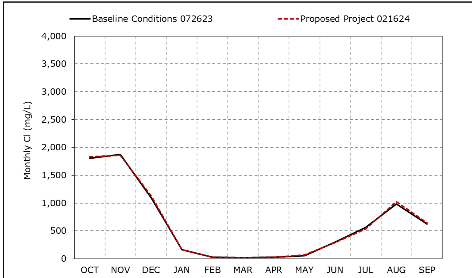
Figure 4B-7-3c. Sacramento River at Collinsville Chloride, Above Normal Year Average CI
