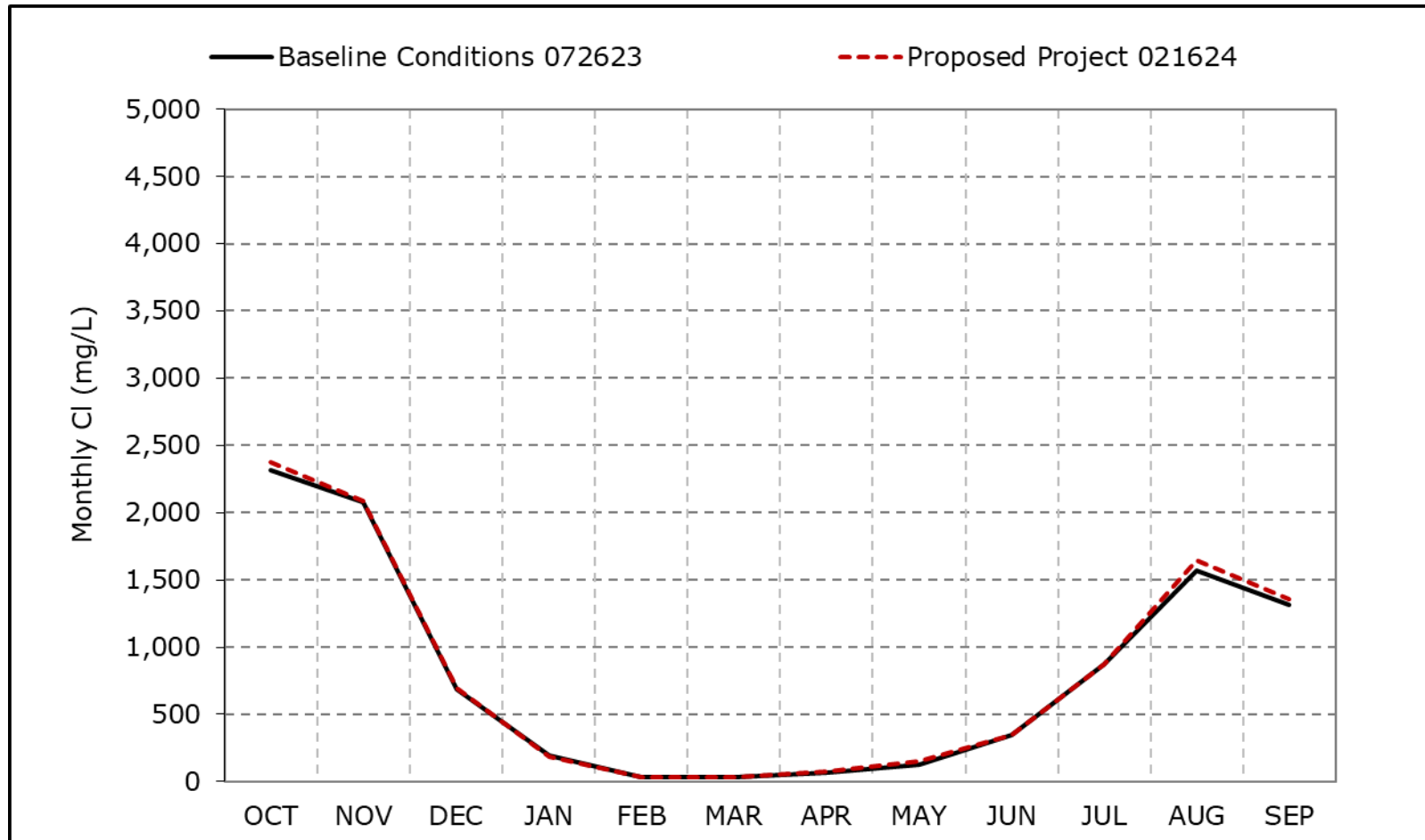
Figure 4B-7-1b. Sacramento River at Mallard Slough Chloride, Wet Year Average Cl
