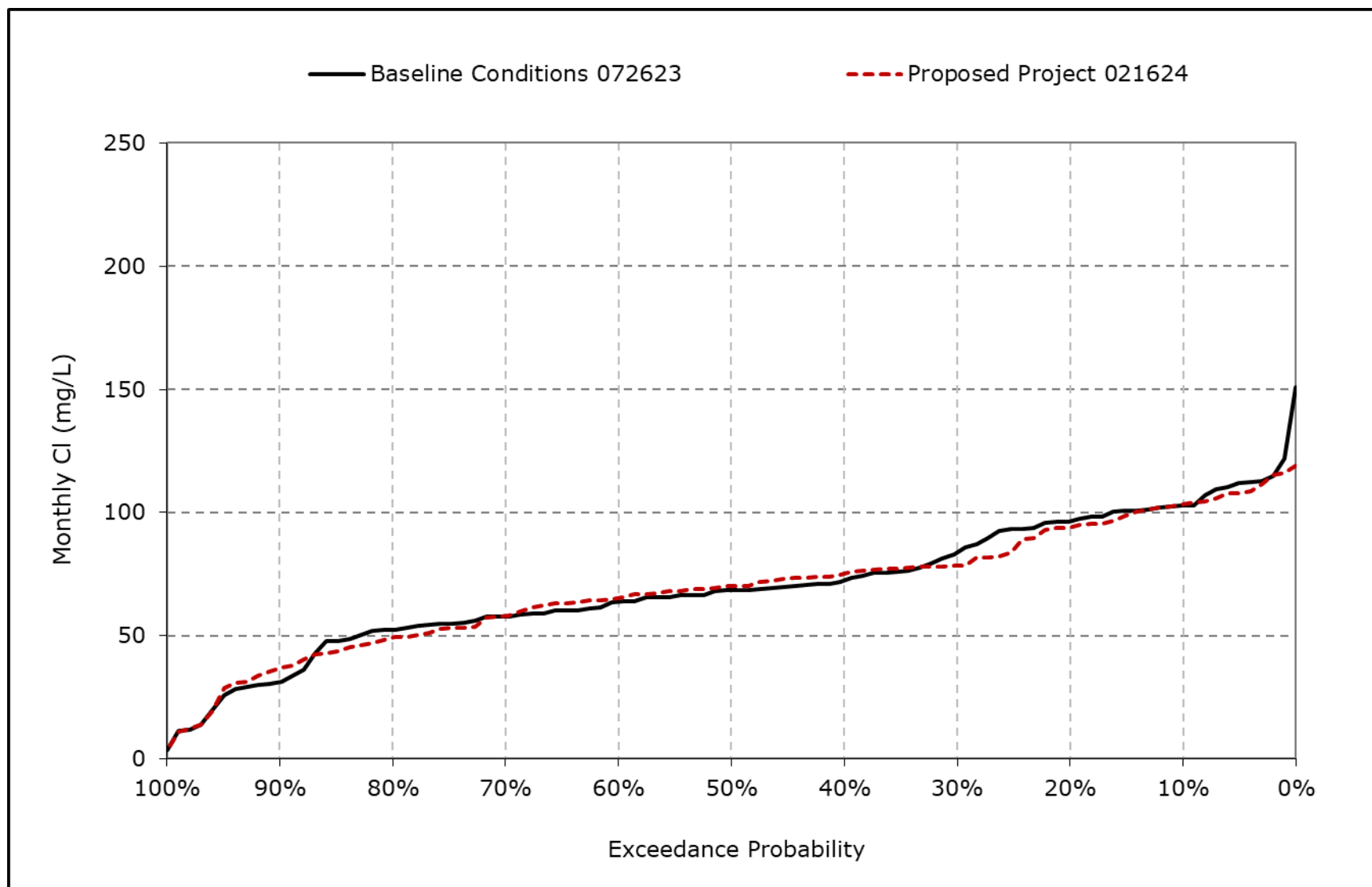
Figure 4B-7-7m. Old River at Highway 4 Chloride, April CI
