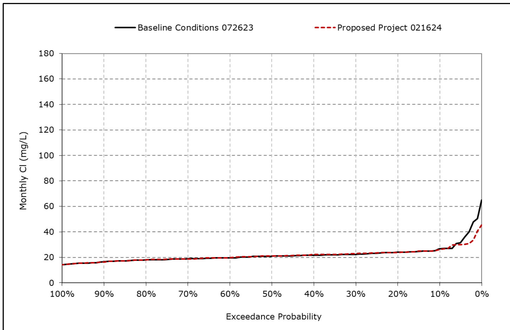
Figure 4B-7-5I. San Joaquin River at San Andreas Chloride, March CI
