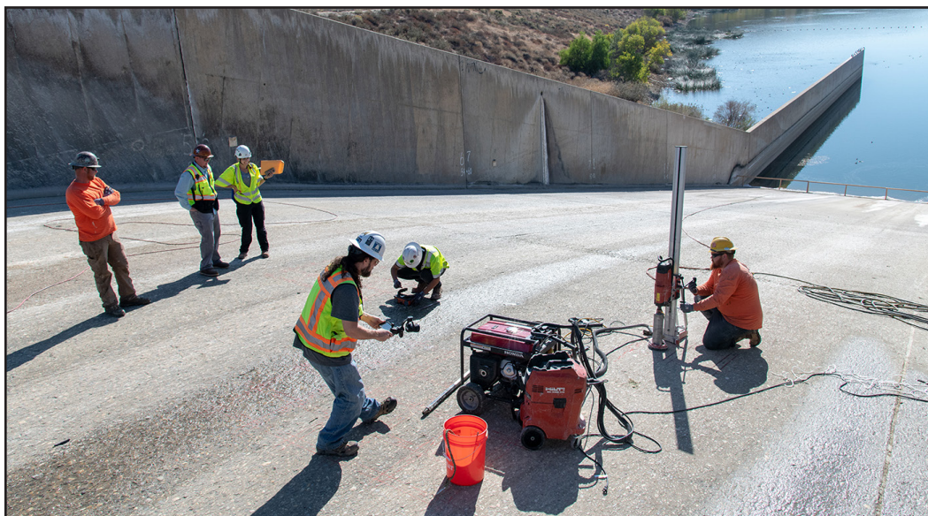
As part of the Castaic Dam Modernization Program, DWR and its contractors take core samples from the Castaic Dam's stream release chute. Castaic Lake State Recreation Area is located in Los Angeles County. Source: Department of Water Resources
