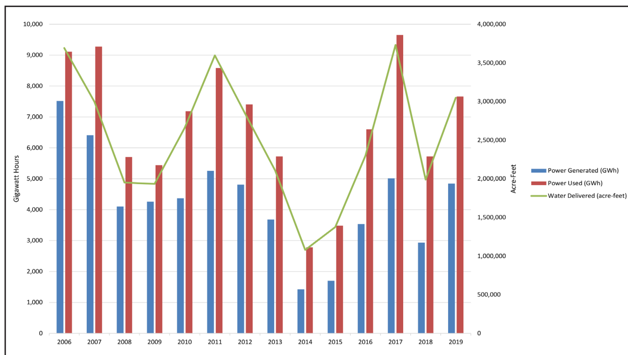
Figure 1: SWP Water Deliveries and Power
